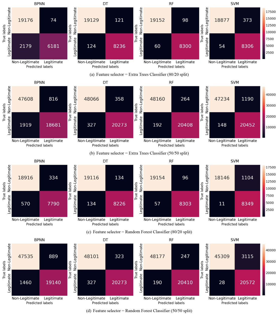
Figure 9: Confusion matrices derived from unbalanced datasets.
