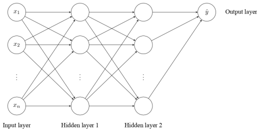
Figure 4: Simplified architecture of the BPNN.
