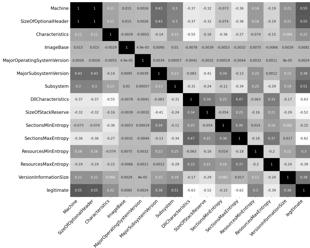
Figure 11: Correlation matrix of features selected by Extra Trees
