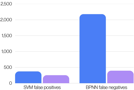
Figure 4. Error counts vs. after class balancing
