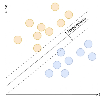
Figure 7: Linear SVM classification
